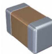
C0603C103J3JACAUTO KEMET CAP CER 10000PF 25V U2J 0603
