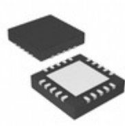
PIC16F720-I/ML Microchip Technology IC MCU 8BIT 3.5KB FLASH 20QFN
