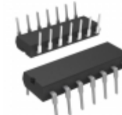
DM74LS11N AMI Semiconductor / ON Semiconductor IC GATE AND 3CH 3-INP 14DIP
