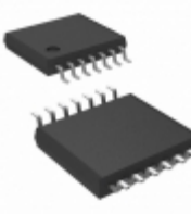
AD5292BRUZ-20-RL7 Analog Devices Inc. IC POT DIG 1024P SPI 20K 14TSSOP
