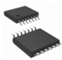
AD5292BRUZ-20 Analog Devices Inc. IC POT DIG 1024P SPI 20K 14TSSOP
