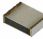
ECW-U1274KC9 Panasonic Electronic Components CAP FILM 0.27UF 10% 100VDC 2820
