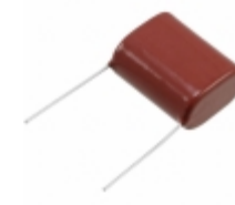
ECQ-E6225KF Panasonic Electronic Components CAP FILM 2.2UF 10% 630VDC RADIAL
