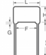
ECQ-P1H561JZ3 Panasonic Electronic Components CAP FILM 560PF 5% 50VDC RADIAL
