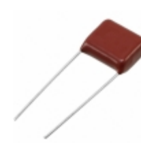
ECQ-E2125JFW Panasonic Electronic Components CAP FILM 1.2UF 5% 250VDC RADIAL
