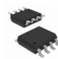
IRF9956TR Infineon Technologies MOSFET 2N-CH 30V 3.5A 8-SOIC
