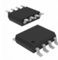
AO4435_102 Alpha & Omega Semiconductor Inc. MOSFET P-CH 30V 10.5A 8SOIC
