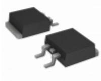
SPB77N06S2-12 Infineon Technologies MOSFET N-CH 55V 80A D2PAK
