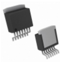
MIC49500WU Microchip Technology IC REG LDO ADJ 5A TO263-7
