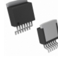
MIC49500-0.9WU Microchip Technology IC REG LDO 0.9V 5A TO263-7
