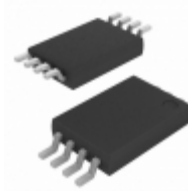
IRF7702 Infineon Technologies MOSFET P-CH 12V 8A 8-TSSOP
