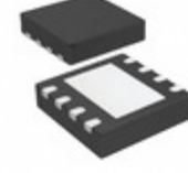
MCP1754ST-3302E/MC Microchip Technology IC REG LDO 3.3V 0.15A 8DFN
