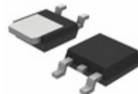
NID5004NT4G ON Semiconductor MOSFET N-CH 40V 6.5A DPAK
