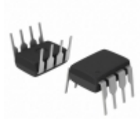
ADM805LAN Analog Devices Inc. IC SUPERVISOR 4.65V WD 8DIP
