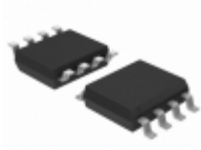
MIC5201-3.0BM Microchip Technology IC REG LDO 3V 0.2A 8SOIC
