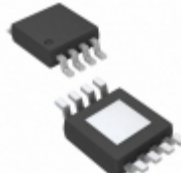
MIC47100-08YMME Microchip Technology IC REG LDO 0.8V 1A 8MSOP
