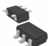
XC6122A218MG-G Torex Semiconductor Ltd IC WATCHDOG TIMER SOT-25
