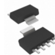
MCP1755T-5002E/DC Microchip Technology IC REG LDO 5V 0.3A SOT223-5
