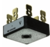
VS-26MT40 Electro-Films (EFI) / Vishay RECTIFIER BRIDGE 400V 25A D- 63
