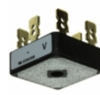
VS-26MT80 Electro-Films (EFI) / Vishay RECTIFIER BRIDGE 800V 25A D- 63
