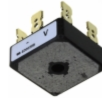
VS-26MT60 Vishay Semiconductor Diodes Division RECTIFIER BRIDGE 600V 25A D- 63
