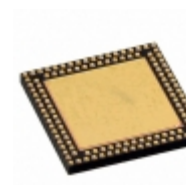
PIC32MZ2048EFG124-E/TL Micrel / Microchip Technology IC MCU 32BIT 2MB FLASH 124VTLA
