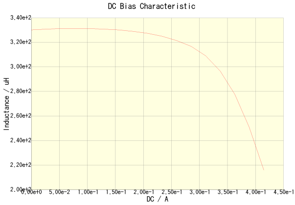
CLF6045T-331M-CA(Amb. Temp. = 20degc)
