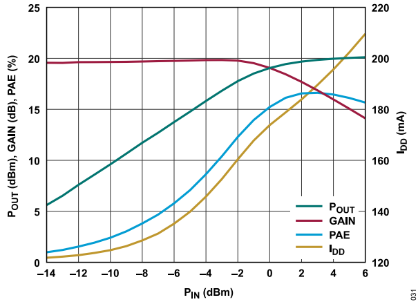
Figure 31. P_{OUT} , Gain, PAE, and I_{DD} vs. P_{IN} , 54 GHz, V_{DD} = 3\text{ V} , I_{DQ} = 120\text{ mA}
