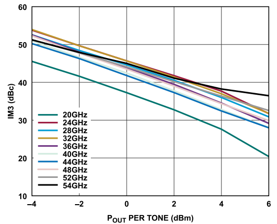
Figure 36. Third-Order Intermodulation Distortion (IM3) vs. P_{OUT} per Tone for Various Frequencies, V_{DD} = 2\text{ V} , I_{DQ} = 120\text{ mA}
