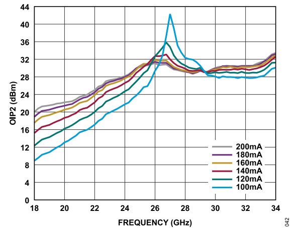
Figure 42. OIP2 vs. Frequency for Various I_{DQ} Values, P_{OUT} per Tone = 0 dBm, V_{DD} = 3 V
