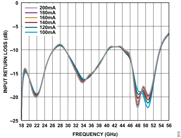
Figure 13. Input Return Loss vs. Frequency for Various I_{DQ} Values, V_{DD} = 3\text{ V}
