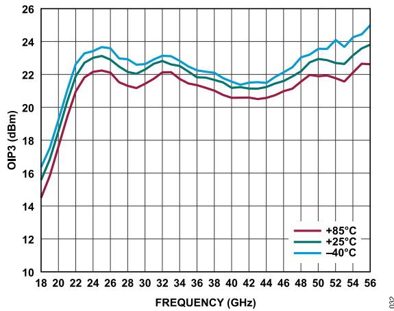
Figure 32. OIP3 vs. Frequency for Various Temperatures, P_{OUT} per Tone = 0 dBm, V_{DD} = 3\text{ V} , I_{DQ} = 120\text{ mA}
