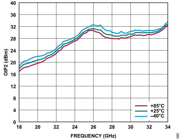
Figure 80. OIP2 vs. Frequency for Various Temperatures, P_{OUT} per Tone = 0 dBm, V_{DD} = 2.5\text{ V} , I_{DQ} = 160\text{ mA}
