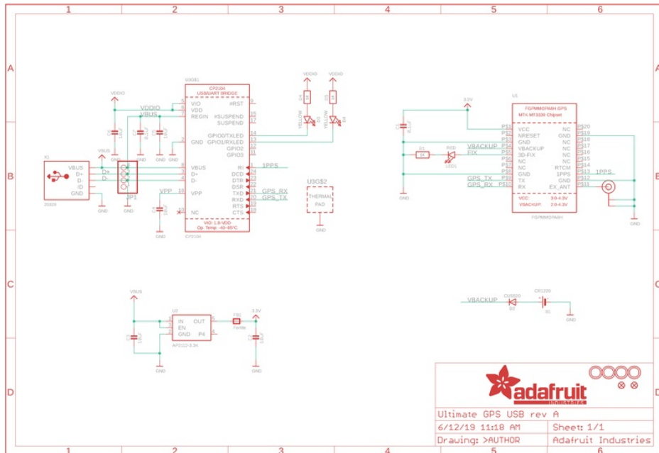
Ultimate GPS USB Fabrication Print
