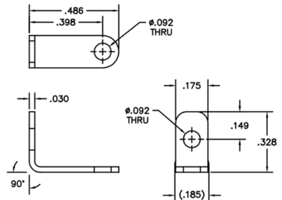
CDG12633 - 2 EACH
