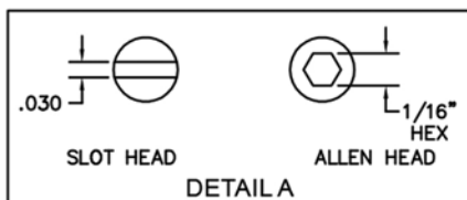
SHORT CAPTIVE JACKSCREW ASSEMBLY JACKSCREW, ALLEN HEAD FACTORY INSTALLED ONLY
