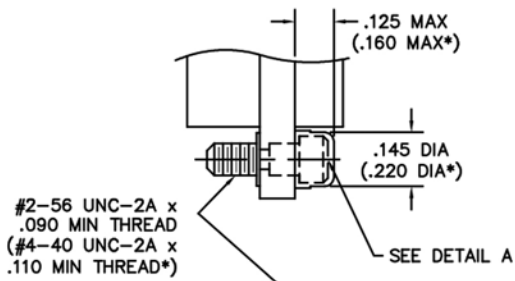
SHORT CAPTIVE JACKSCREW ASSEMBLY JACKSCREW, ALLEN HEAD FACTORY INSTALLED ONLY
