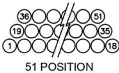
CONNECTOR MATING FACE (RECEPTACLE)
