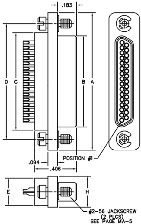
PLUG
