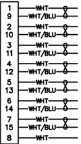
15 POSITION
