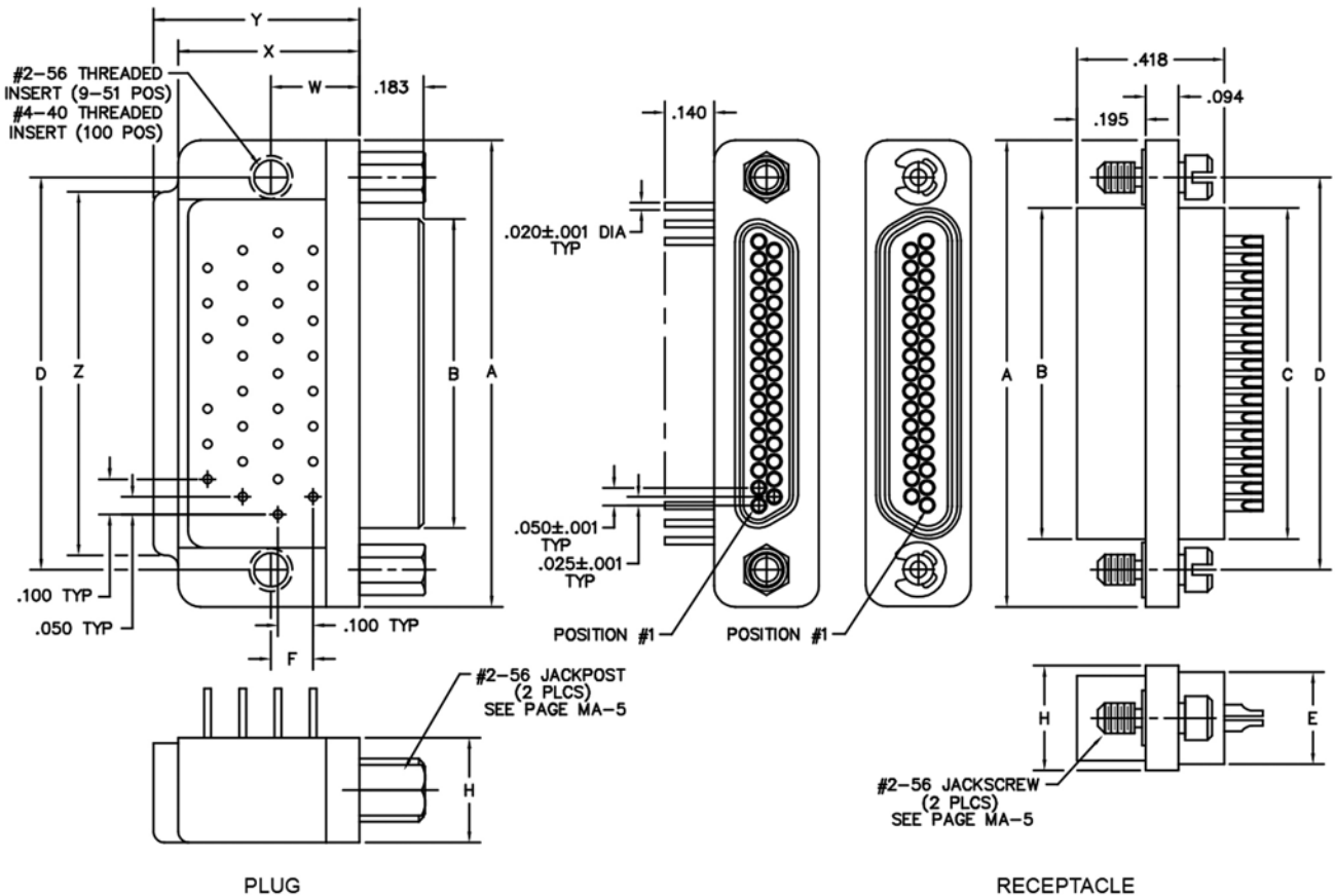
PLUG
