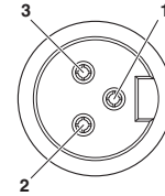
Pin assignment, socket, 7/8"-16UNF, 3-pos., view of female side
