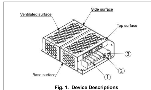
Fig. 1. Device Descriptions
