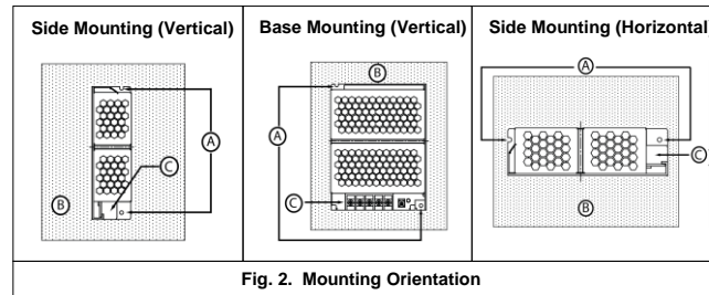
Fig. 2. Mounting Orientation
