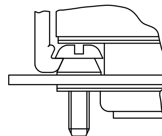
Rear mounted connector example
