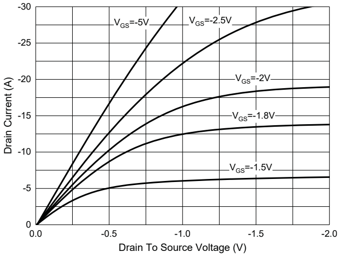
Fig. 7 - Output Characteristics
