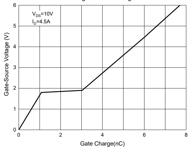
Fig. 4 - Gate Charge
