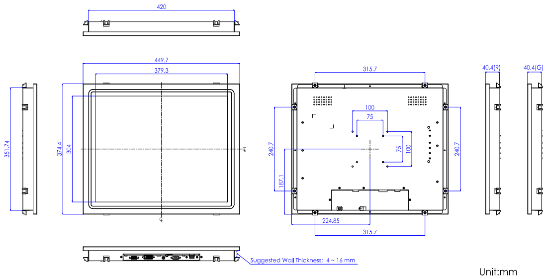
Figure 2.1 IDS-3219 Series Dimensions
