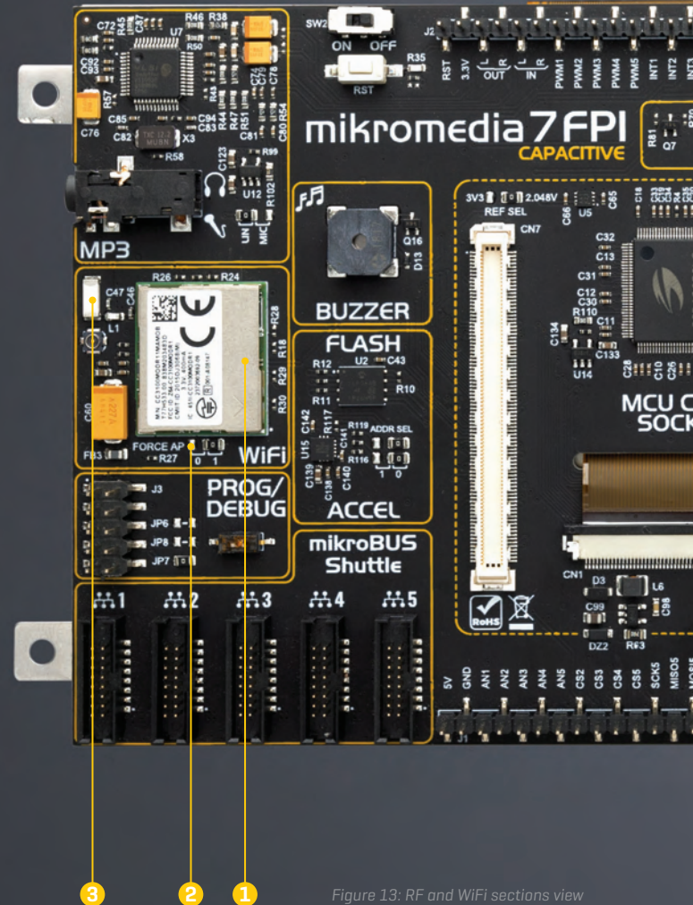
Figure 13: RF and WiFi sections view
