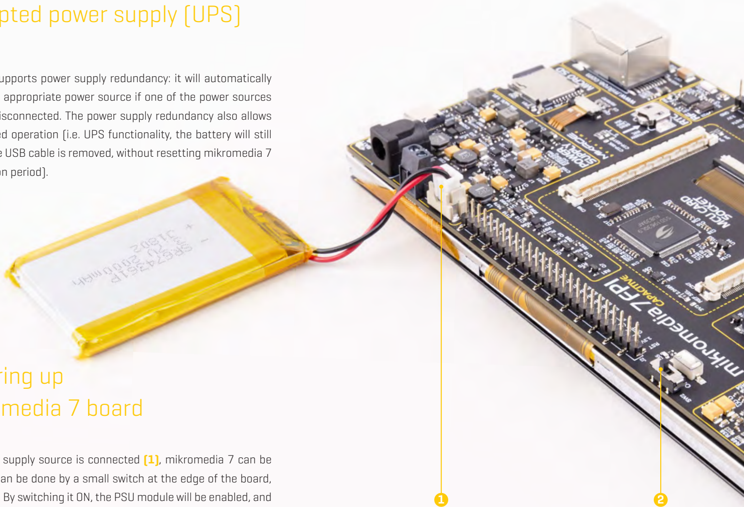
Figure 8: Battery power supply connection view
