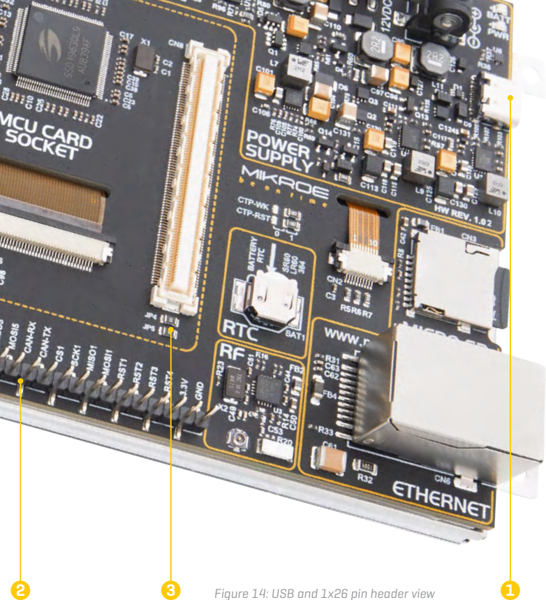
Figure 14: USB and 1x26 pin header view
