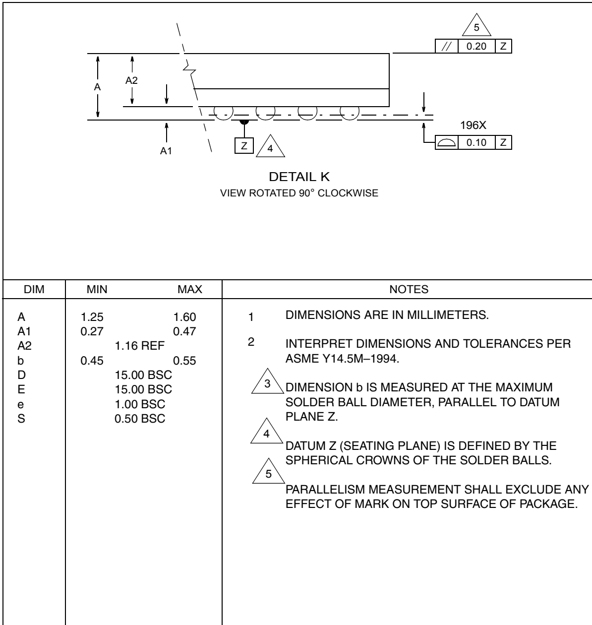
Figure 8-2. 196 MAPBGA Dimensions
