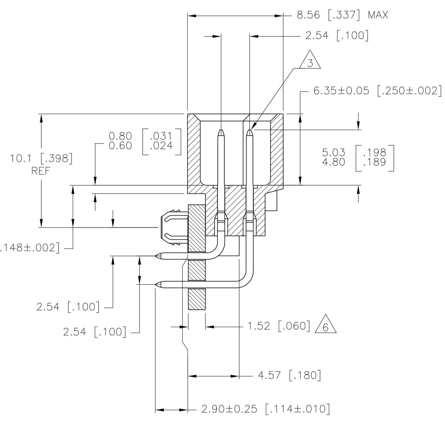
SECTION Z-Z
