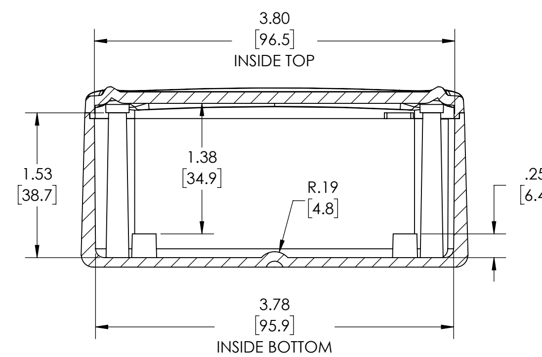
SECTION B-B
