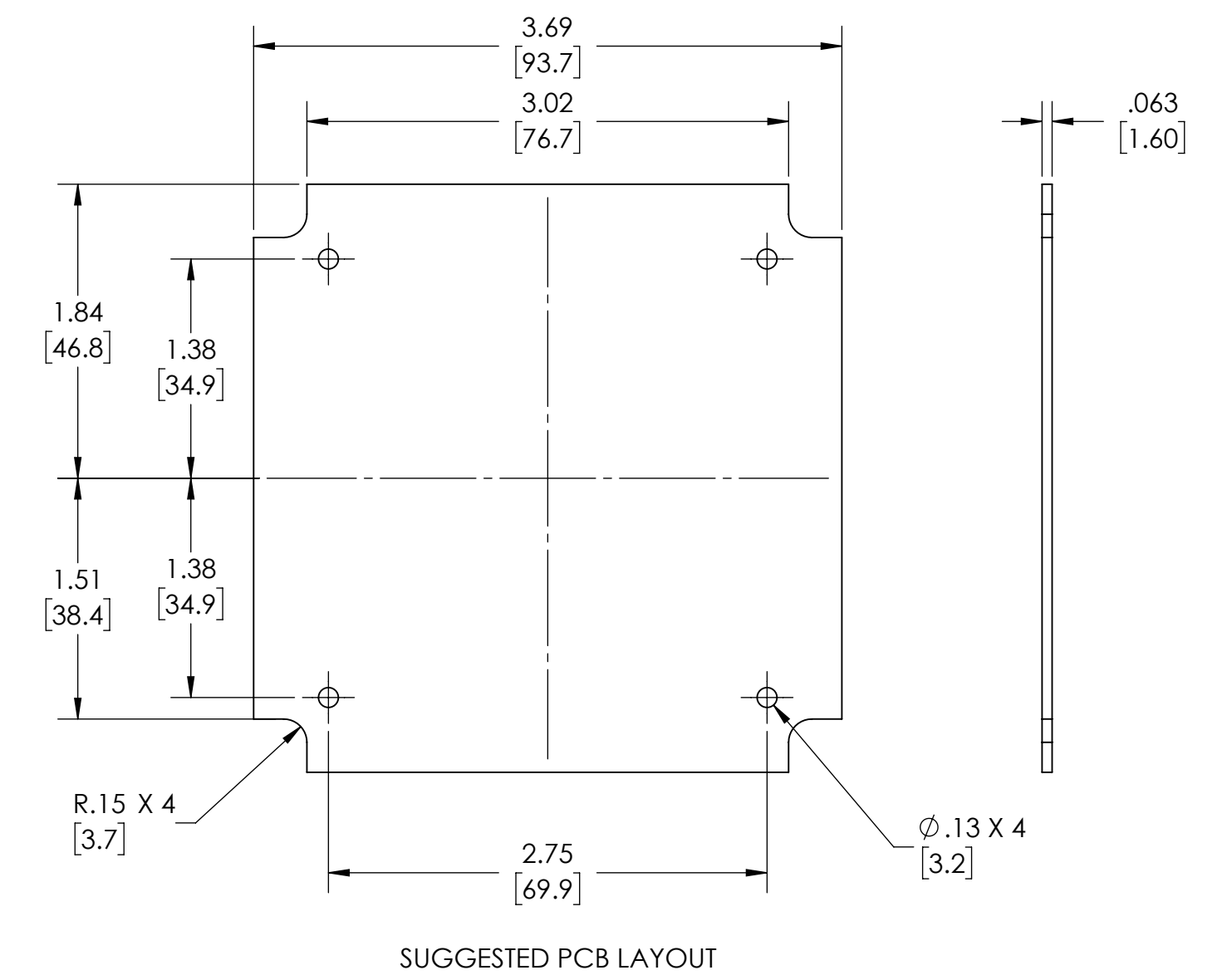
SUGGESTED PCB LAYOUT
