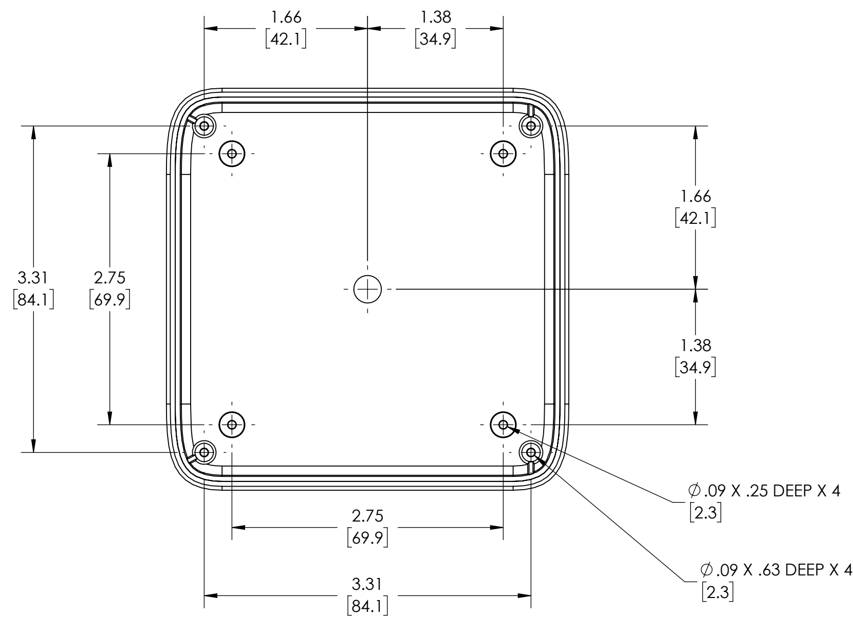
INSIDE VIEW OF BODY COVER NOT SHOWN
