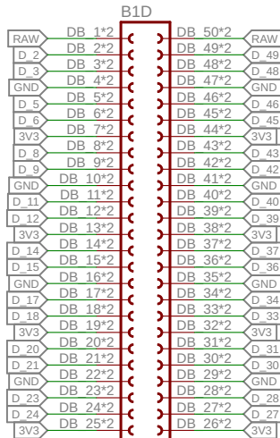
ALCHITRY_SHIELD
