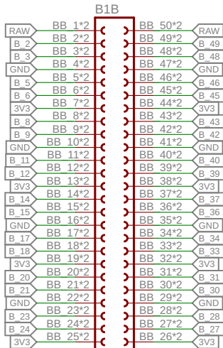
ALCHITRY_SHIELD
