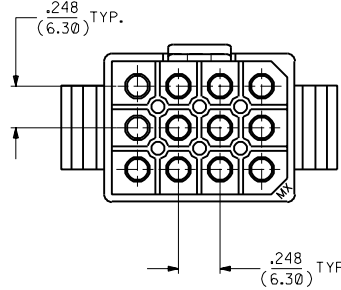
PLUG
