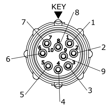
WIRING END W8882-9PG-P-5XX
