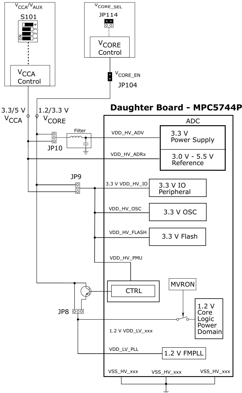
Figure 5. Power Supplies - Configuration of the Mother Board
