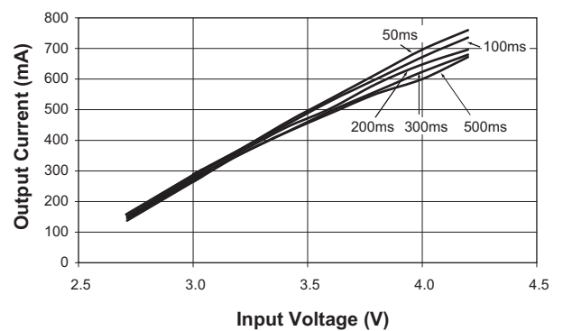
Output Current vs. Input Voltage ( 70^\circ C ) ( V_{OUT} > 4.5V )
