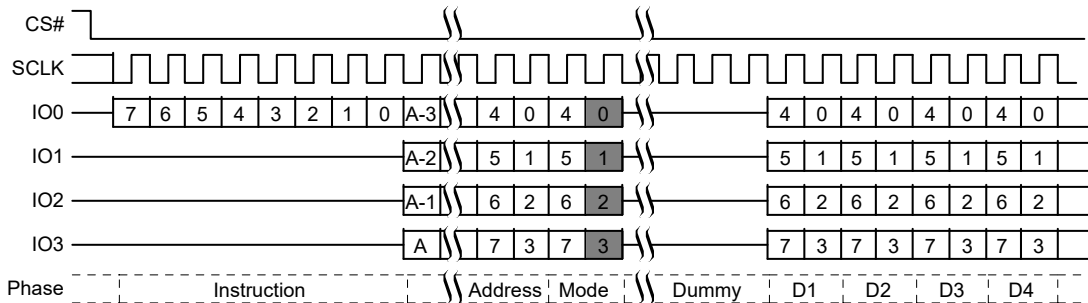
Figure 71. Quad I/O Read Initial Access Command Sequence [36]
