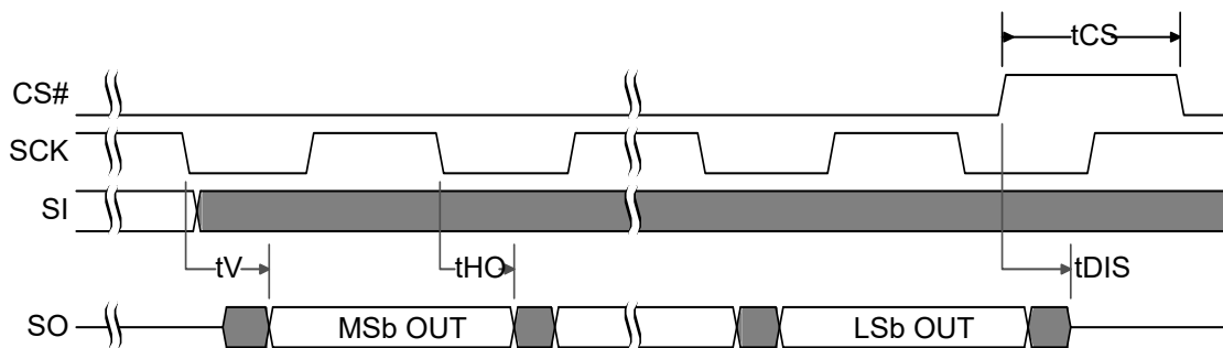
Figure 144. SPI Single Bit Output Timing
