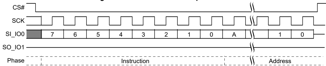
Figure 99. IBUL Command Sequence [56, 57]
