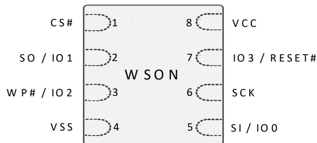
Figure 4. 8-Connector Package (WSO5N 5 x 6), Top View [3]
