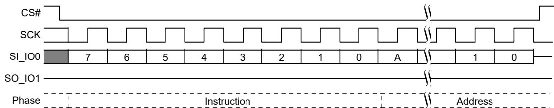
Figure 82. Half Block Erase (HBE 52h or 4HBE 53h) Command Sequence [46, 47]
