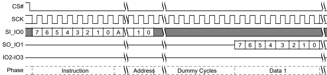
Figure 66. Fast Read (FAST_READ) Command Sequence
