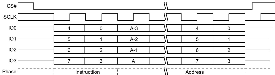
Figure 83. Half Block Erase (HBE 52h or 4HBE 53h) QPI Mode Command Sequence [46, 47]
