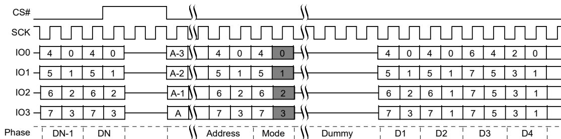
Figure 73. Continuous Quad I/O Read Command Sequence [36, 38]
