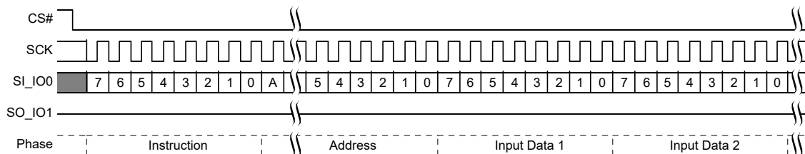
Figure 77. Page Program (PP 02h or 4PP 12h) Command Sequence [42]
