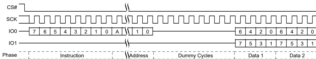
Figure 67. Dual Output Read Command Sequence [32]
