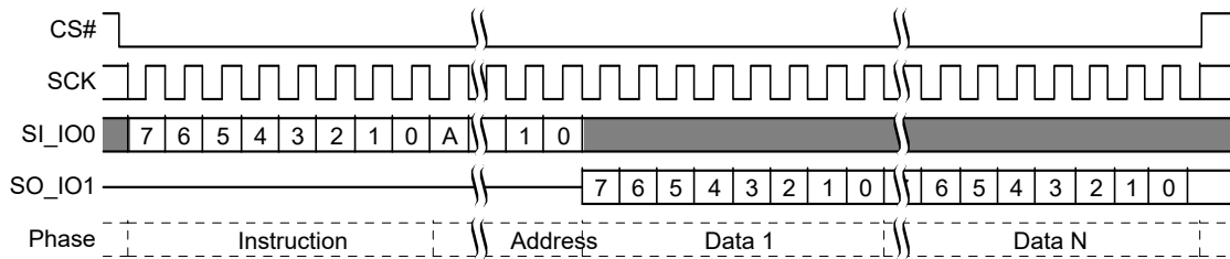
Figure 65. Read Command Sequence [31]
