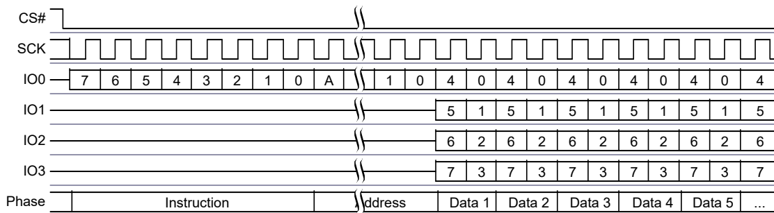
Figure 79. Quad Page Program Command Sequence [44]
