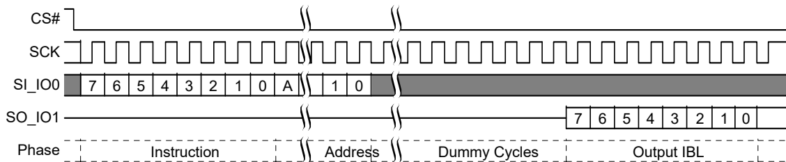
Figure 95. IBLRD Command Sequence [52, 53]
