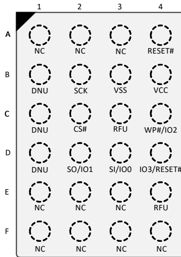
Figure 6. 24-Ball BGA, 4 x 6 Ball Footprint (FAC024), Top View [5]
