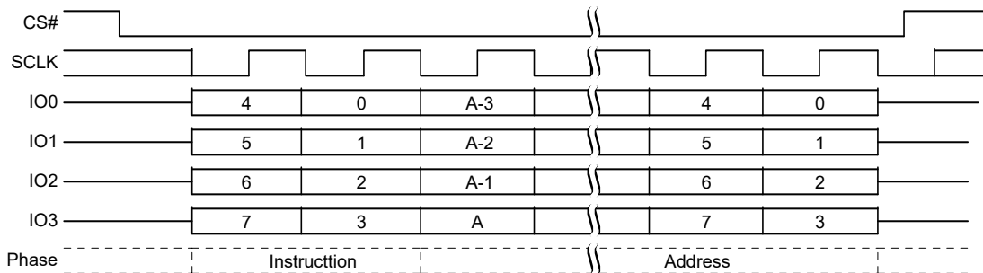
Figure 100. IBUL Command Sequence QPI Mode [58, 59]
