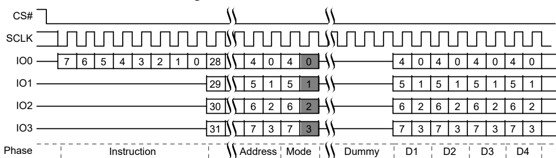
Figure 20. Quad I/O Command [7]
