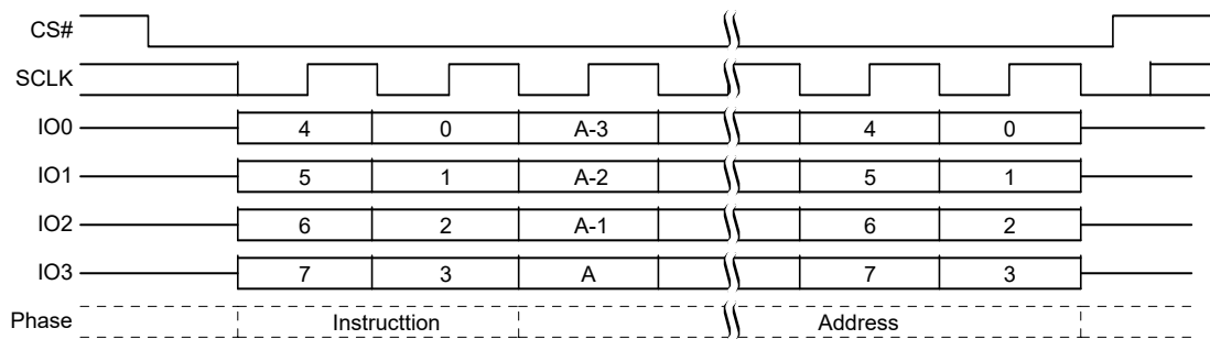
Figure 81. Sector Erase (SE 20h or 4SE 21h) QPI Mode Command Sequence [45]
