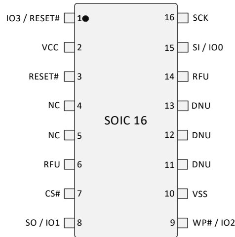
Figure 1. 16-Lead SOIC Package (SO3016), Top View
