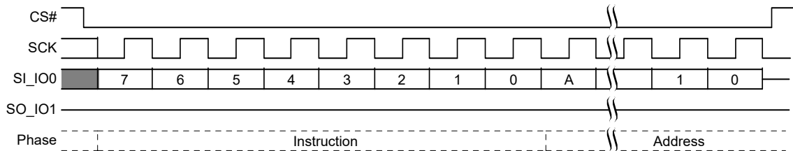
Figure 80. Sector Erase (SE 20h or 4SE 21h) Command Sequence [45]
