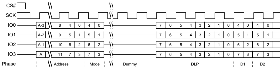
Figure 76. Continuous DDR Quad I/O Read Subsequent Access [39, 40, 41]
