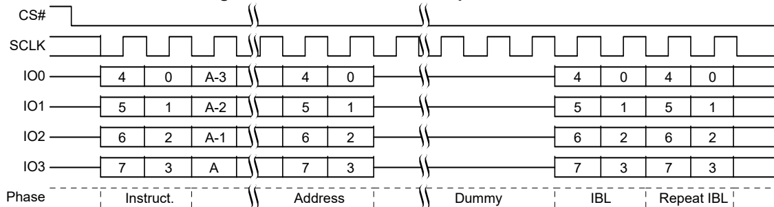
Figure 96. IBLRD Command Sequence QPI [52, 53]
