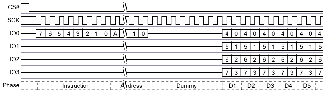
Figure 68. Quad Output Read Command Sequence [33]
