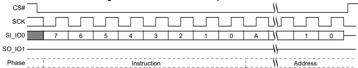
Figure 105. SPRP Command Sequence [60, 61]
