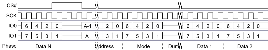
Figure 70. Dual I/O Continuous Read Command Sequence [34]
