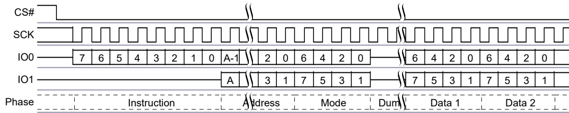
Figure 70. Dual I/O Continuous Read Command Sequence [34]
