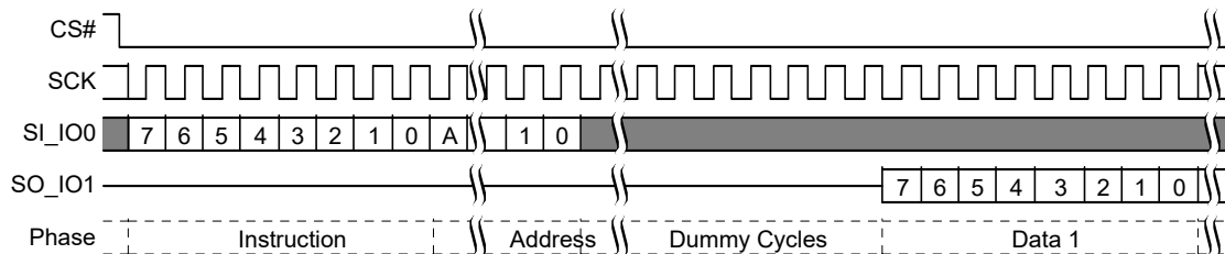
Figure 93. Security Regions Read Command Sequence [50]
