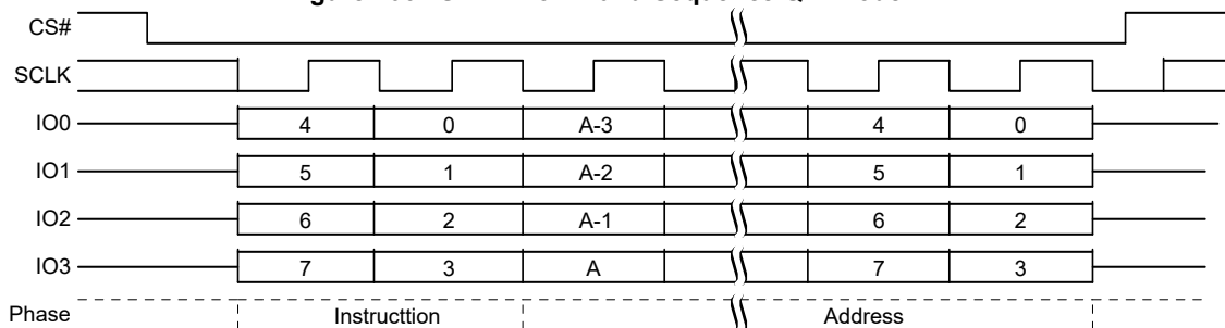
Figure 106. SPRP Command Sequence QPI Mode [60, 61]
