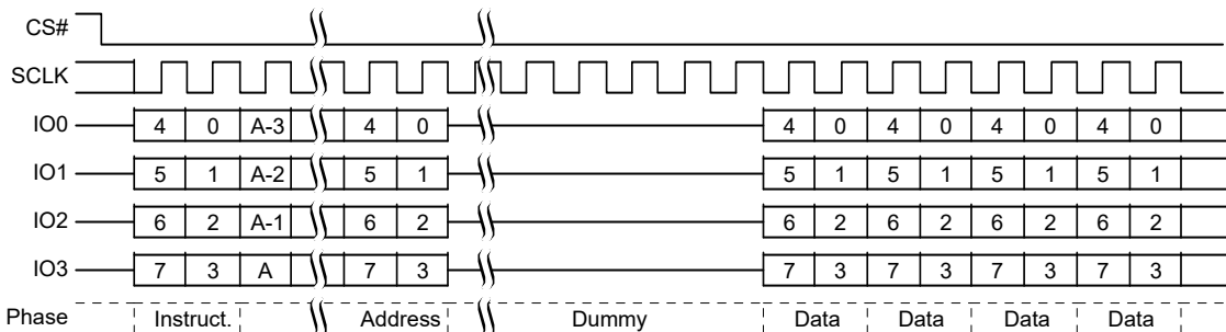
Figure 60. Read Any Register, QPI Mode, Command Sequence [30]
