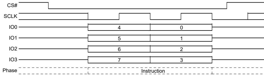
Figure 102. Global IBL Lock (GBL) Command Sequence QPI Mode
