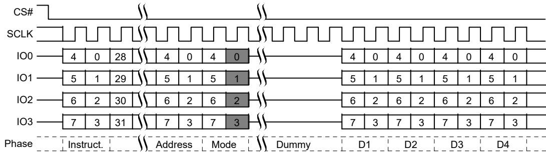
Figure 21. Quad I/O Read Command in QPI Mode [8]
