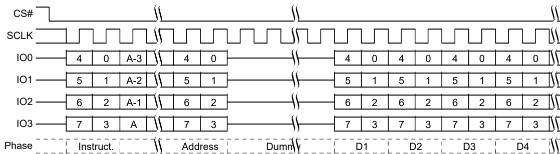
Figure 94. Security Regions Read Command Sequence QPI Mode [51]
