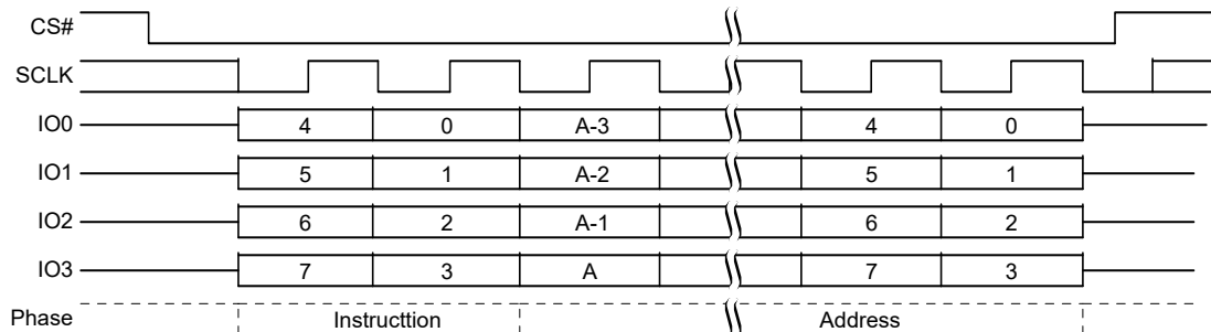
Figure 85. Block Erase (BE D8h or 4BE DCh) QPI Mode Command Sequence [48]
