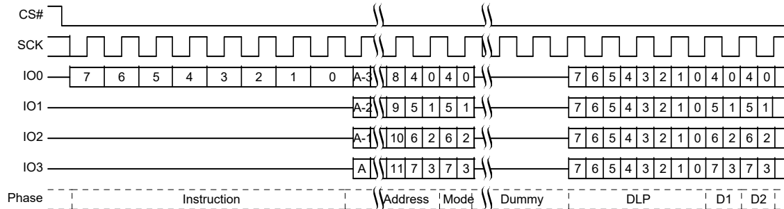
Figure 74. DDR Quad I/O Read Initial Access [39, 40]
