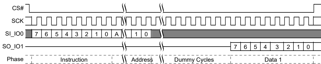
Figure 31. RSFDP Command Sequence [29]
