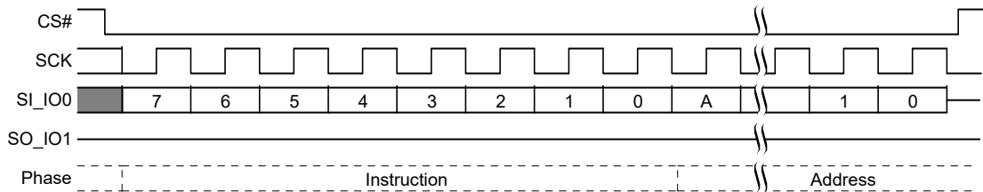
Figure 84. Block Erase (BE D8h or 4BE DCh) Command Sequence [48]
