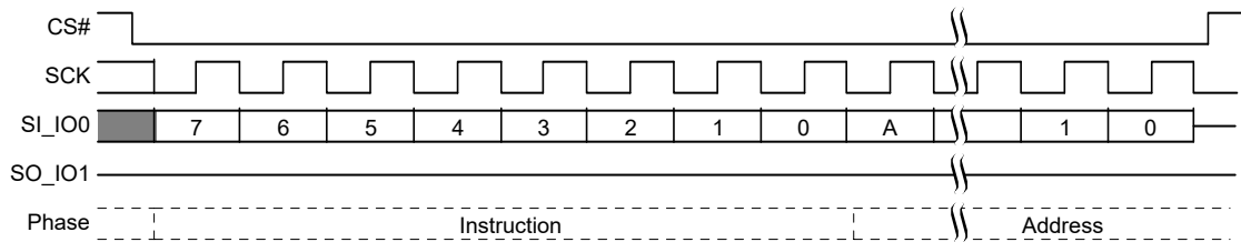
Figure 97. IBL Command Sequence [54, 55]
