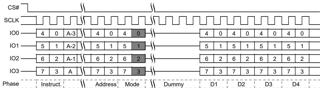
Figure 73. Continuous Quad I/O Read Command Sequence [36, 38]
