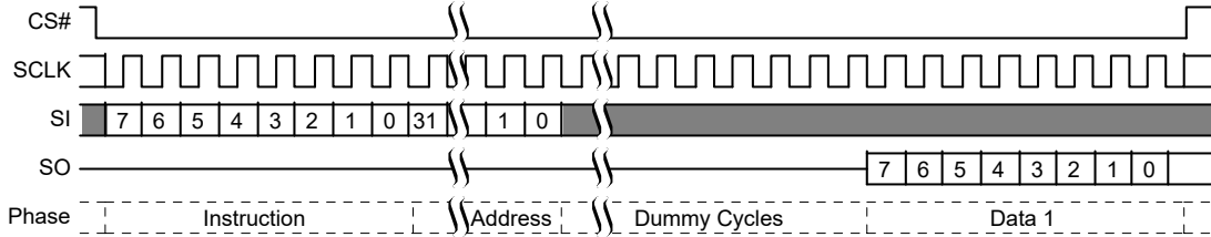
Figure 16. Single Bit Wide I/O Command with latency
