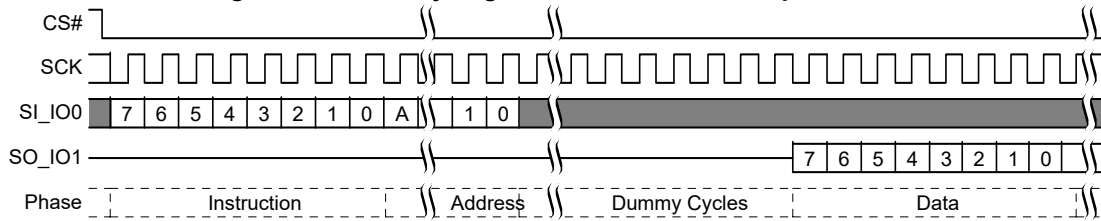
Figure 59. Read Any Register Read Command Sequence [30]
