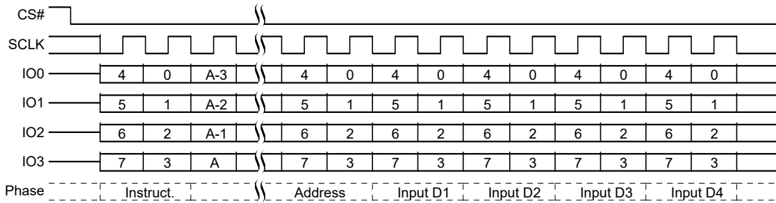
Figure 78. Page Program (PP 02h or 4PP 12h) QPI Mode Command Sequence [43]
