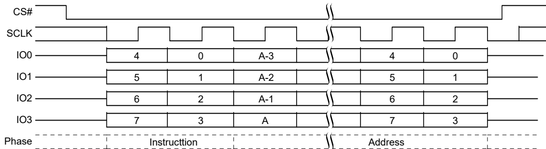
Figure 98. IBL Command Sequence QPI Mode [54, 55]
