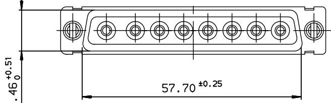
LAYOUT DIMENSIONS (after plating) CONNECTOR SIDE VIEW
