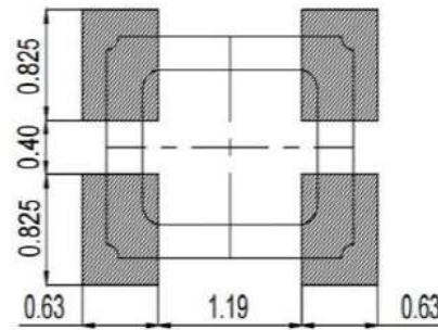
Figure 2) Land Pattern
