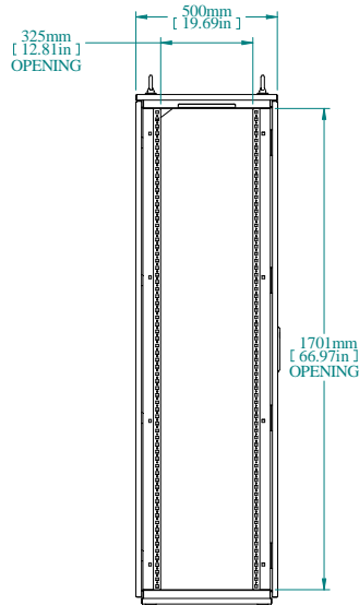
L.S. VIEW
