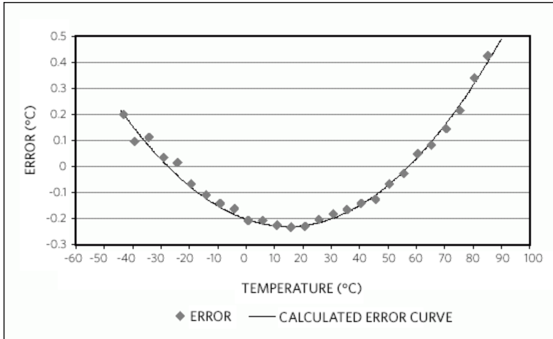
Figure 1. DS1631 measured error and calculated error.
