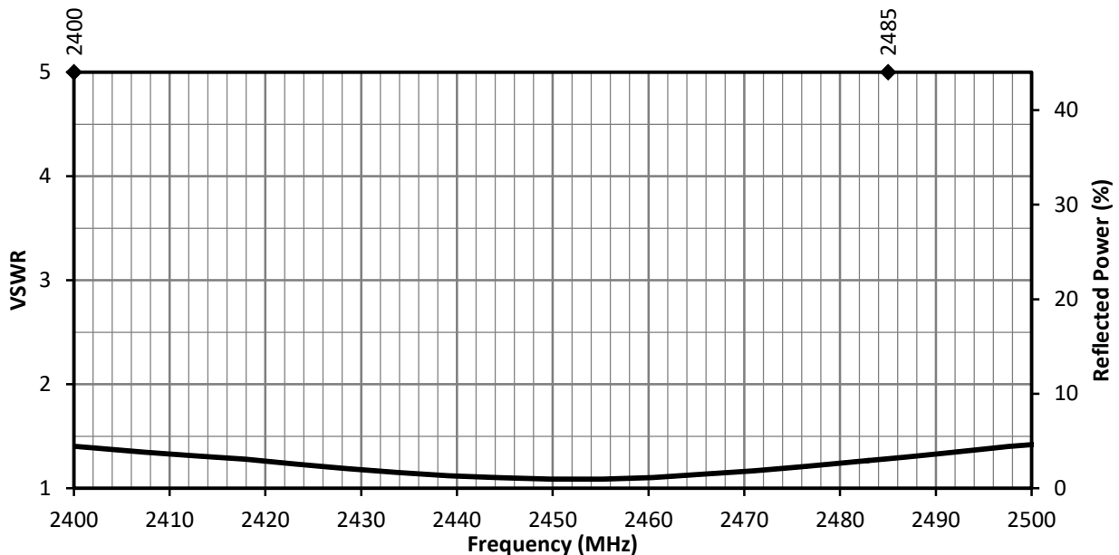
Figure 2. ANT-2.4-FPC-SH Antenna VSWR
