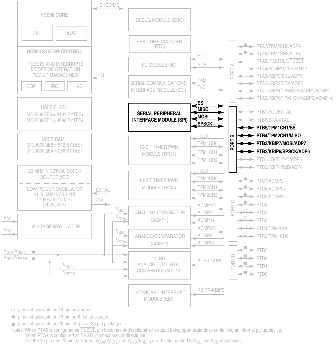
Figure 15-1. MC9S08QE8 Series Block Diagram Highlighting SPI Block and Pins
