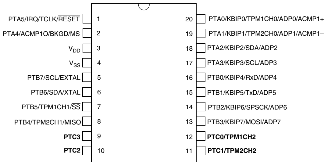
Figure 2-3. MC9S08QE8 Series in 20-Pin SOIC Package
