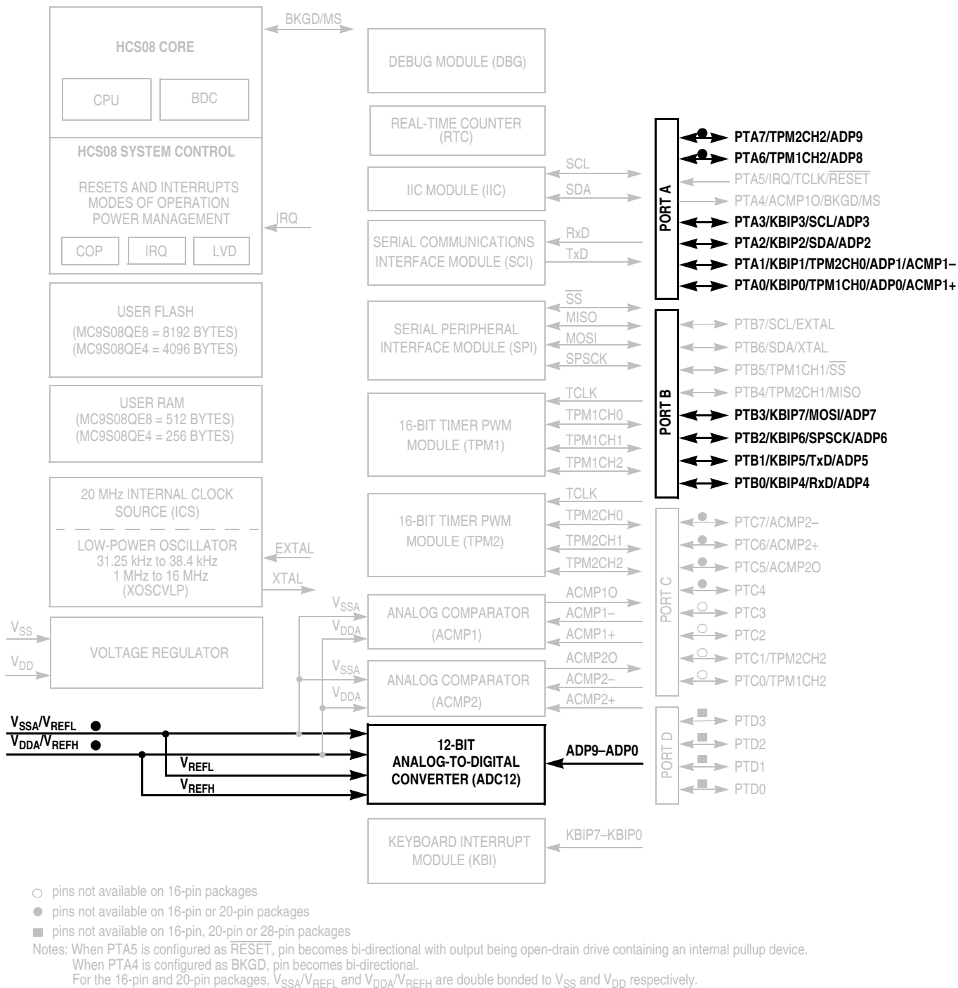
Figure 10-1. MC9S08QE8 Series Block Diagram Highlighting ADC Block and Pins
