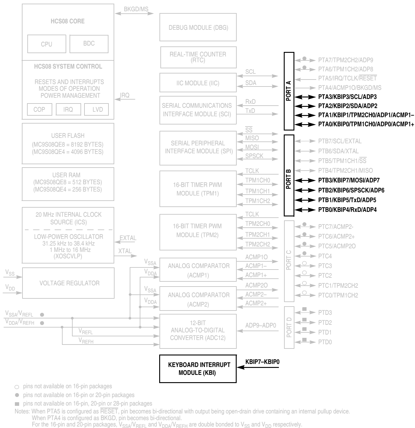
Figure 7-1. MC9S08QE8 Series Block Diagram Highlighting KBI Block and Pins
