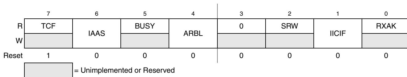
Figure 12-6. IIC Status Register (IICS)
