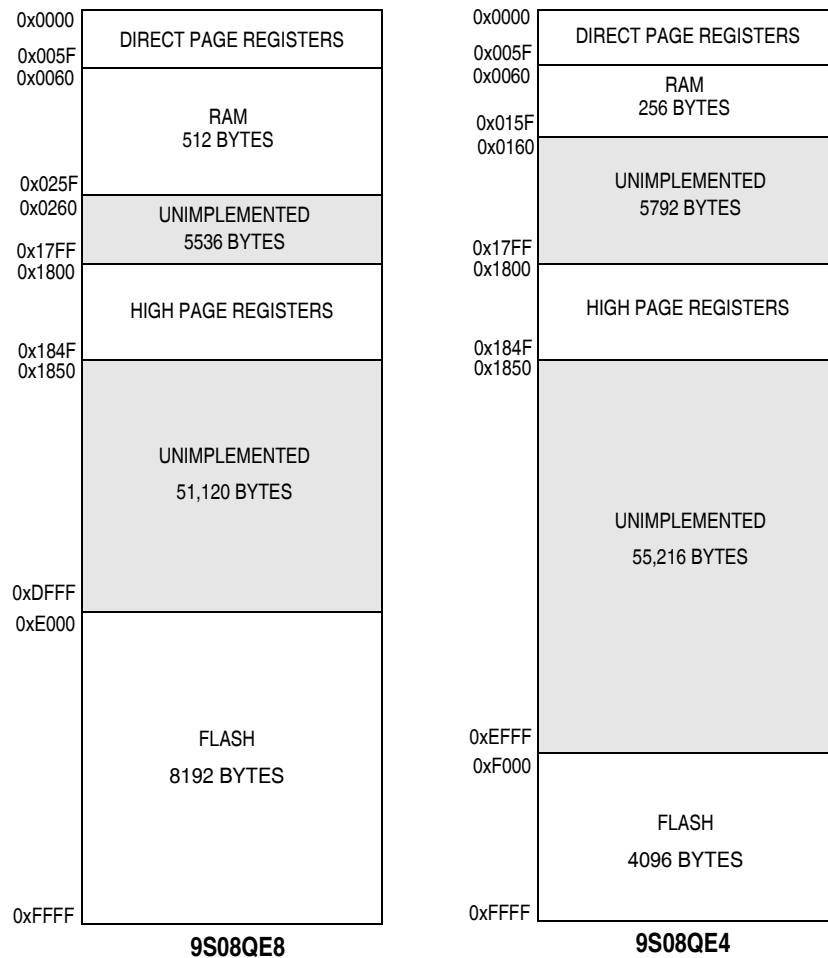
Figure 4-1. MC9S08QE8 Series Memory Maps
