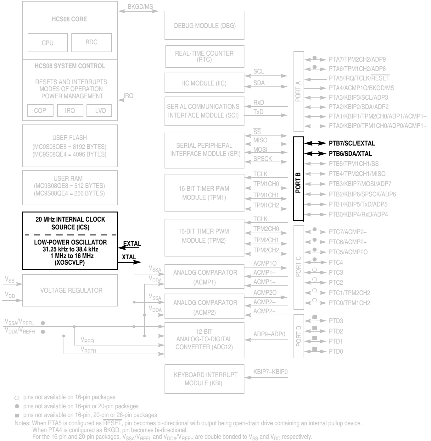
Figure 11-1. MC9S08QE8 Series Block Diagram Highlighting ICS Block and Pins
