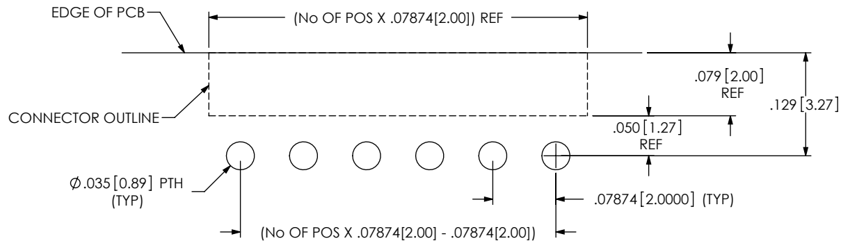
FIG 1 TMMH-1XX-XX-S-RA SHOWN
