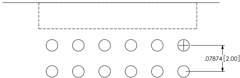
FIG 2 TMMH-1XX-XX-D-RA SHOWN SAME AS FIG 1, EXCEPT AS SHOWN
