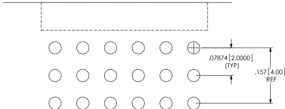
FIG 3 TMMH-1XX-XX-T-RA SHOWN SAME AS FIG 1, EXCEPT AS SHOWN
