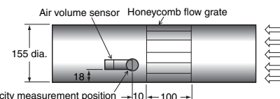
Figure 2: Wind Tunnel
