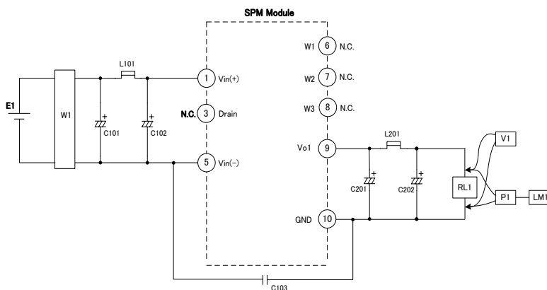
Measurement circuit
